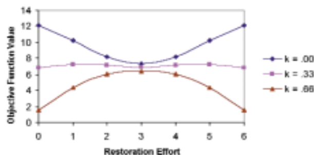
Figure 5. E(A+B) - kV(A+B) — small budget case
