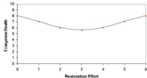
Figure 7. Maximin strategy — small budget
